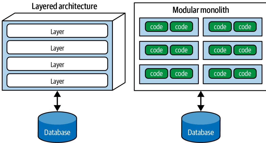
Figure 9-2. Two types of top-level partitioning: technical (such as the layered architecture) and domain (such as the modular monolith)
